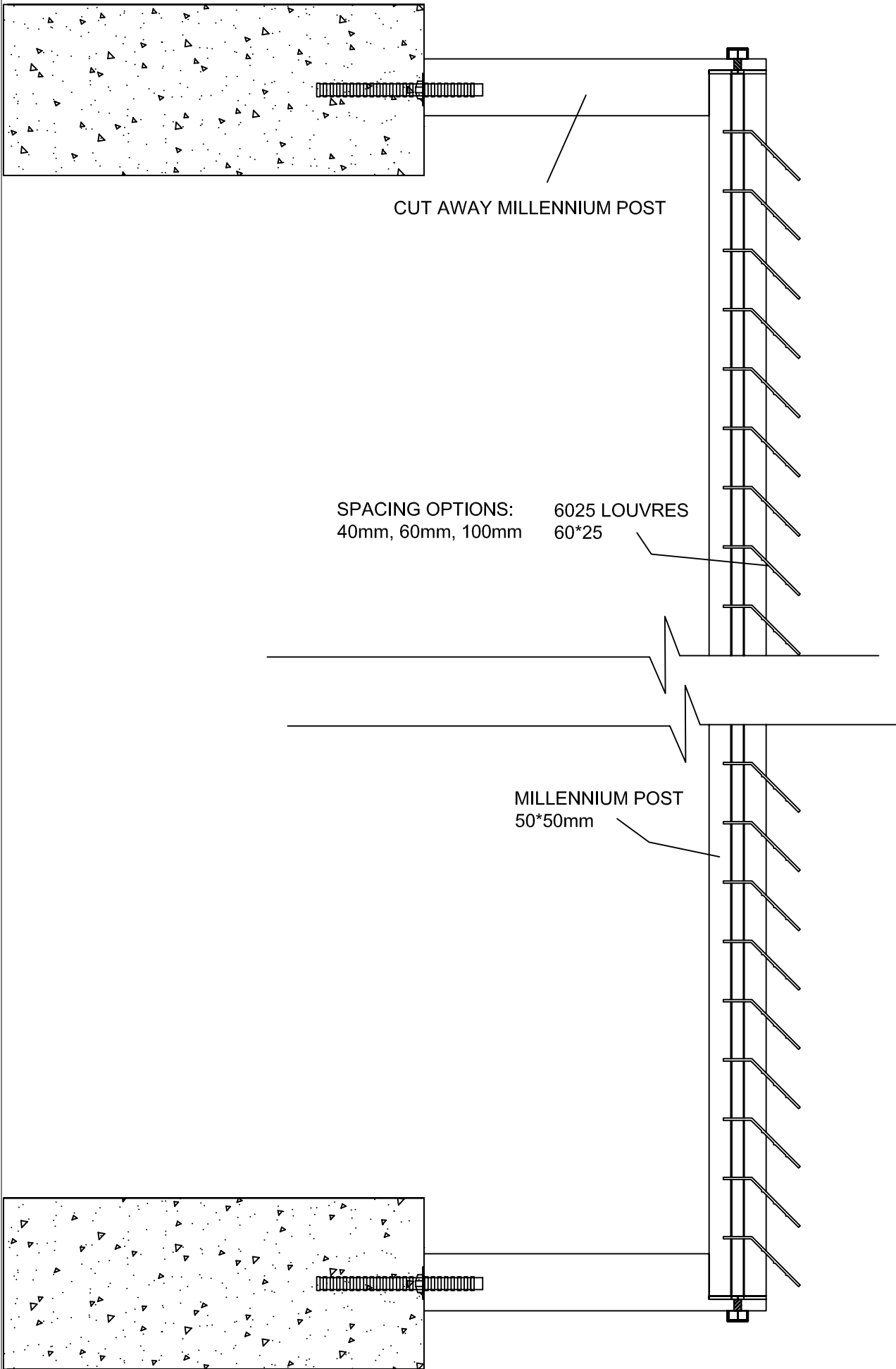
6025 LOUVRES FACE-FIXED WITH MILLENNIUM POST
